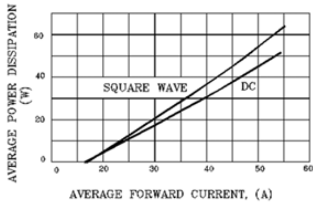
FIG.4. FORWARD POWER DISSIPATION
